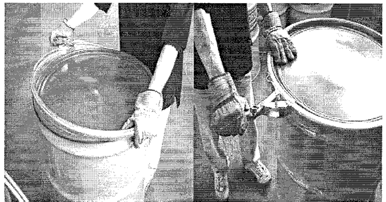
Figure 7 – Expanded ring being placed on drum
